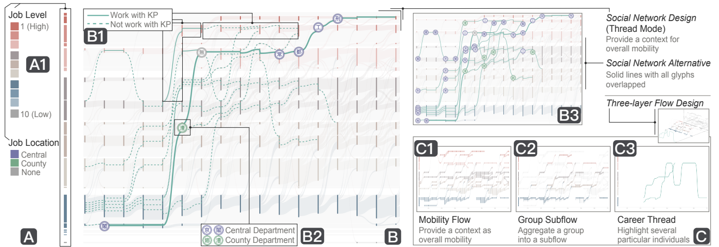
Fig. 3. The visual design of CareerLens . (A) The color legend used in two job-level and department flows. (B) The CareerFlow View visualizes the overall career mobility using an enhanced Sankey diagram. (B1) and (B2) are the detailed design components and (B3) is a component alternative in CareerFlow View. (C) The three-layer flow design in Population Flow , including individual thread, group subflow, and overall mobility flow.
