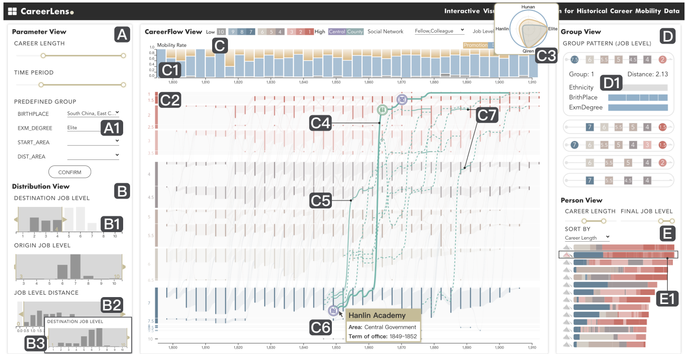
Fig. 2. The system interface of CareerLens . The Parameter View (A) provides several constraints for specifying a target population. The Distribution View (B) displays the job level summary for filtering interested individuals. The CareerFlow View (C) presents the mobility patterns in two parts: (1) a percent stacked bar chart showing mobility evolution and a glyph comparing the group features and (2) an enhanced flow showing mobility in job-level and department modes. The Group View (D) and Person View (E) list latent groups and influential individuals respectively for comparison.
