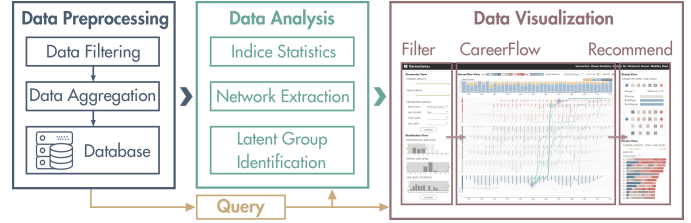
Fig. 1. System overview. CareerLens has three parts: a data preprocessing module, a data analysis module, and a data visualization module.
